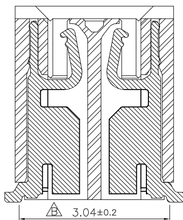
A-A cross section Scale : X2
