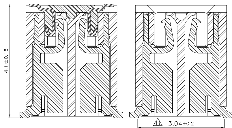
Matting drawing
