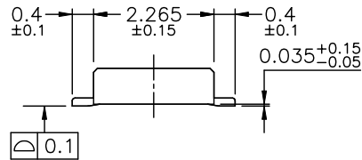
MATED DRAWING(REF.)
