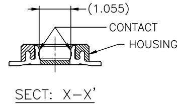
MATED DRAWING(REF.)
