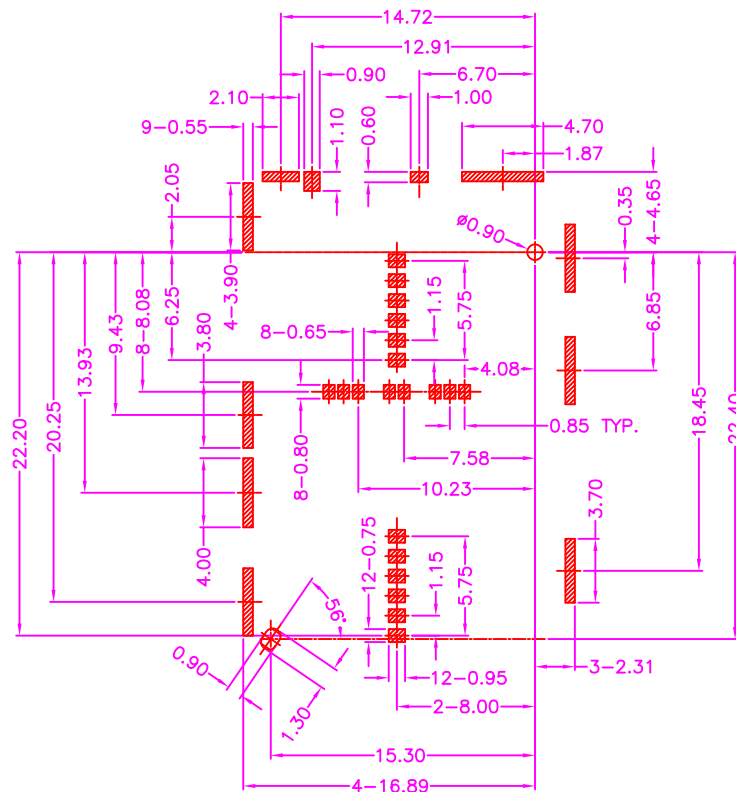
P.C.B LAYOUT TOP VIEW ±0.05
