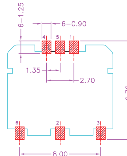
P.C.B LAYOUT TOP VIEW ±0.05
