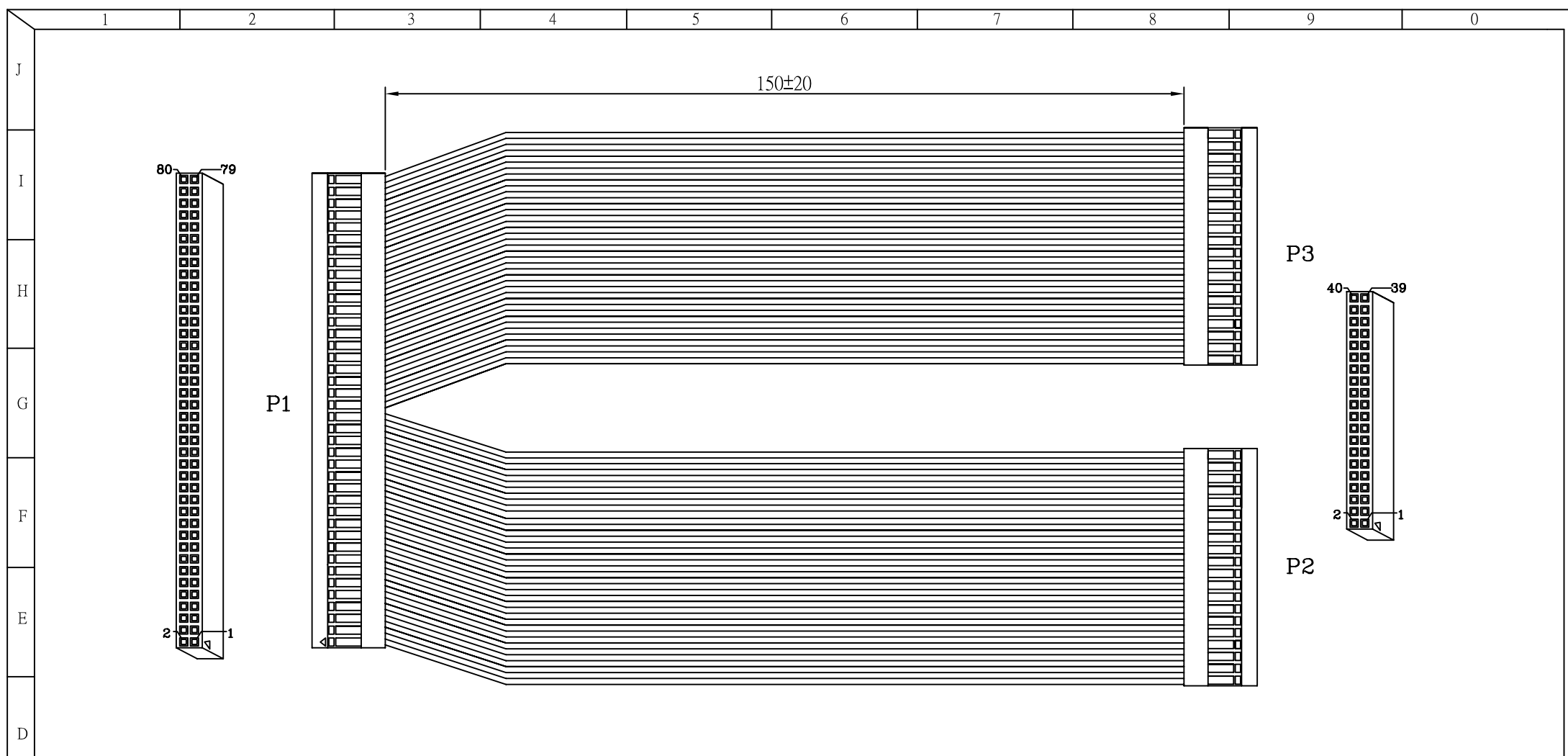
WIRING DIAGRAM
