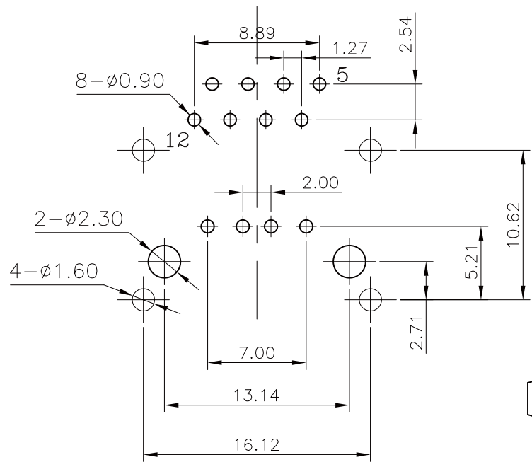
PCB LAYOUT/TOP VIEW
