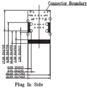
Keep-Out Area (Component Side View):
