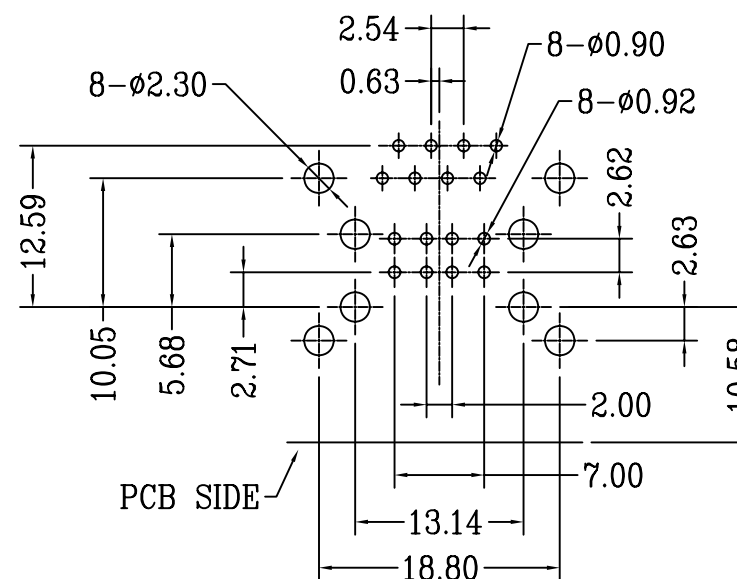
PCB LAYOUT
