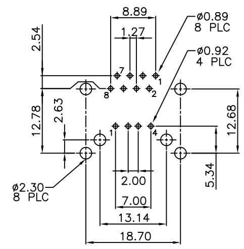
PCB LAYOUT Ref.
