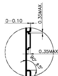
DETAIL A
