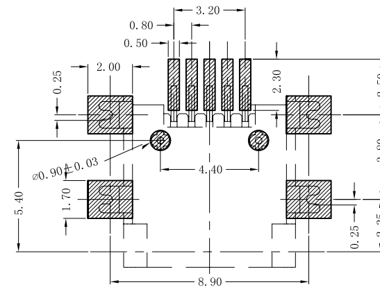
FIGURE A:PRINTED CIRCUIT BOARD (PCB) layout
