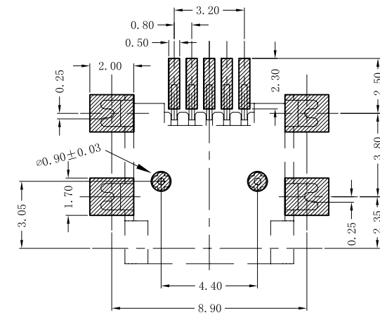
FIGURE A:PRINTED CIRCUIT BOARD (PCB) layout
