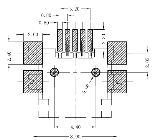
FIGURE A: PRINTED CIRCUIT BOARD (PCB) layout
