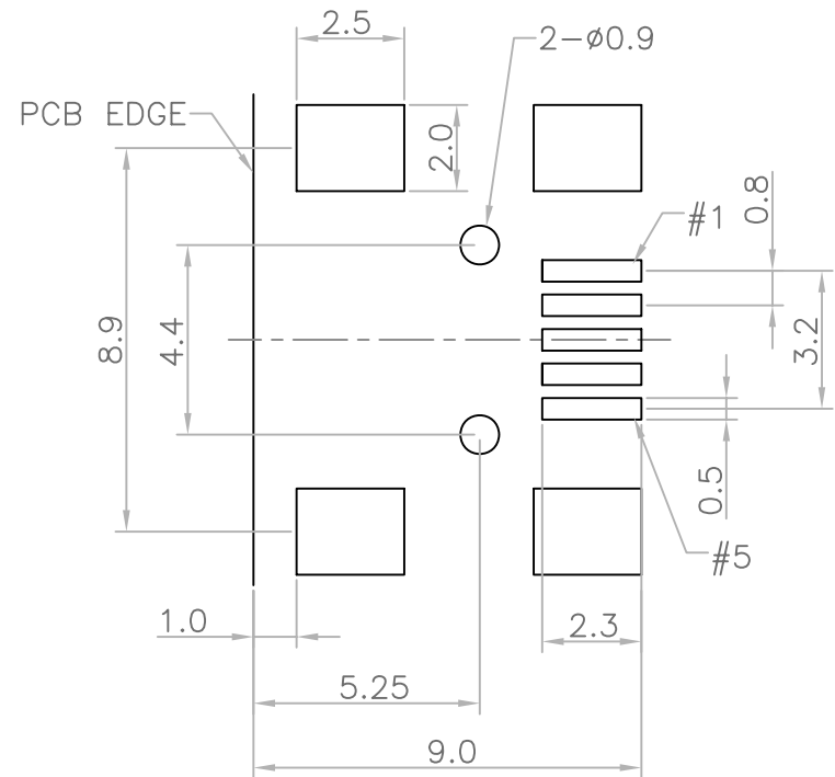
PCB LAYOUT
