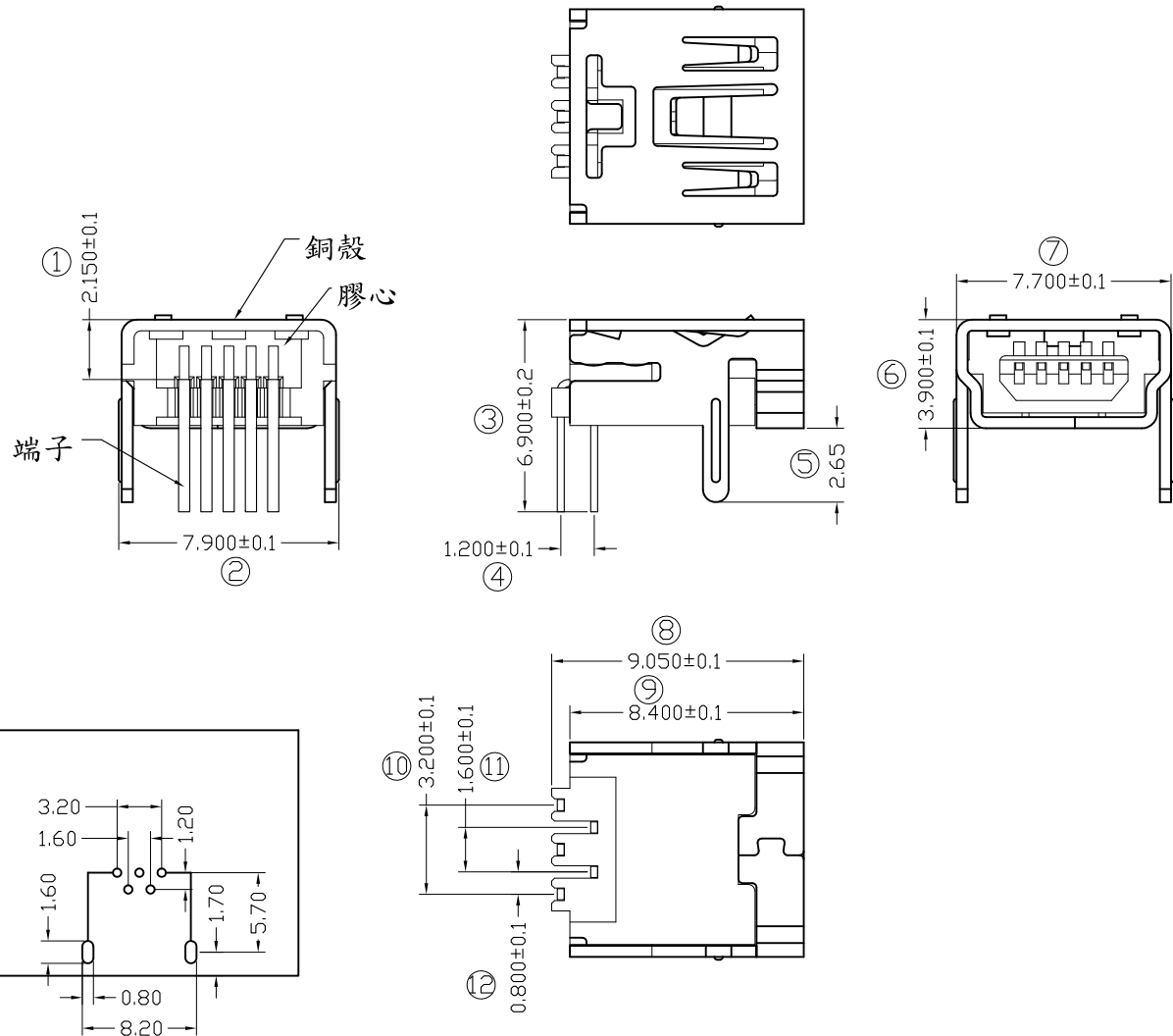
P.C.B. LAYOUT SCALE 2.00
