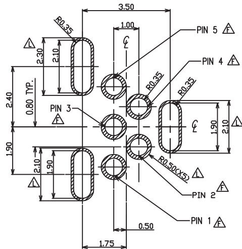
FIGURE A : Printed Circuit Board (PCB) Layout(scale 10 : 1)
