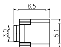
HOUSING + PIN
