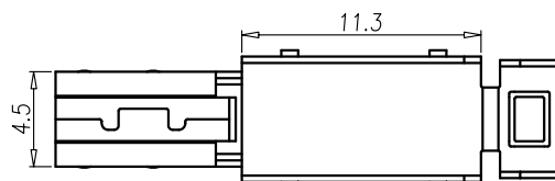
FRONT SHELL
