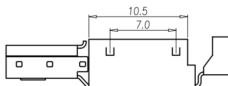
BACK SHELL
