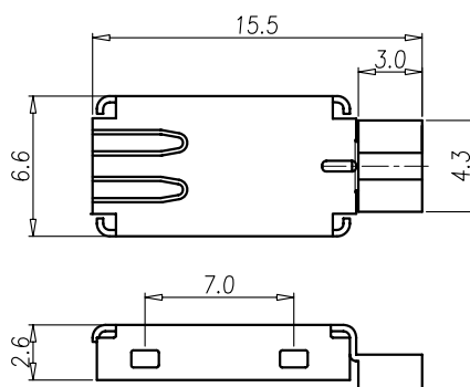
FRONT SHELL
