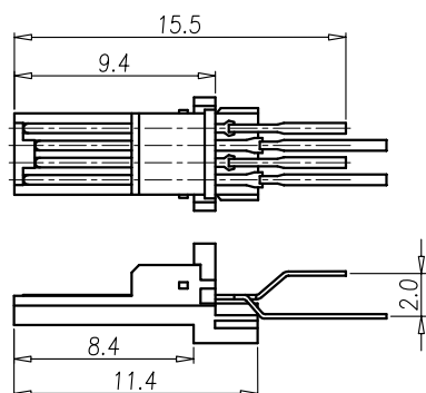
HOUSING + PIN
