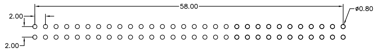
Recommended P.C.B Layout
