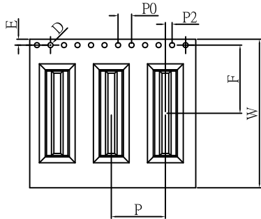
TAPE TYPE 1 : FOR POSITION NUMBERS 04 THRU 10(TAPE WIDTH < 32mm)
