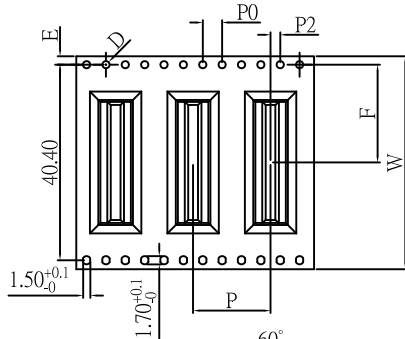
TAPE TYPE 2 : FOR POSITION NUMBERS 12 AND ABOVE(TAPE WIDTH ≥ 32mm)
