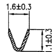
B-B SECTION
