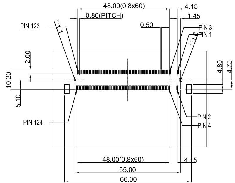
RECOMMEND PC BOARD LAYOUT
