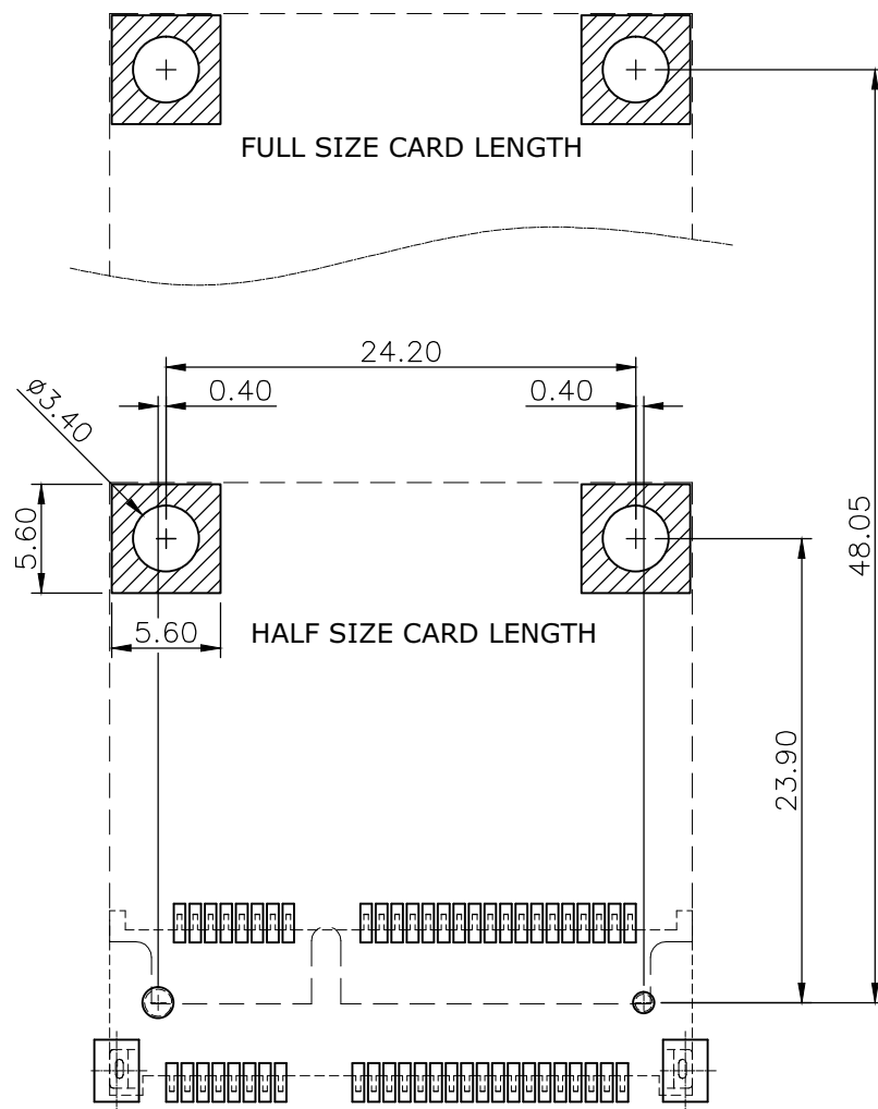
RECOMMEND LAYOUT (TOP VIEW)
