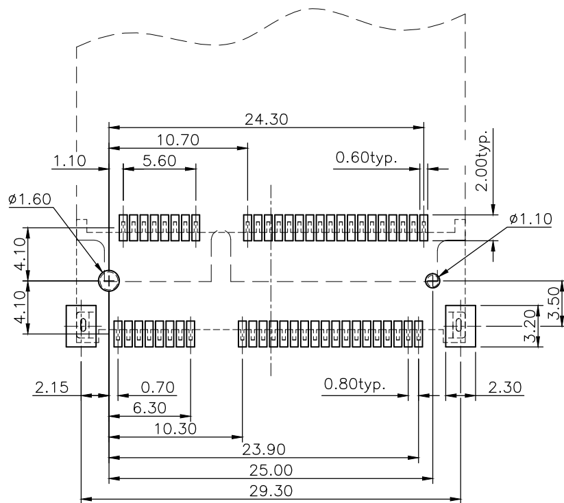
RECOMMEND LAYOUT (TOP VIEW)
