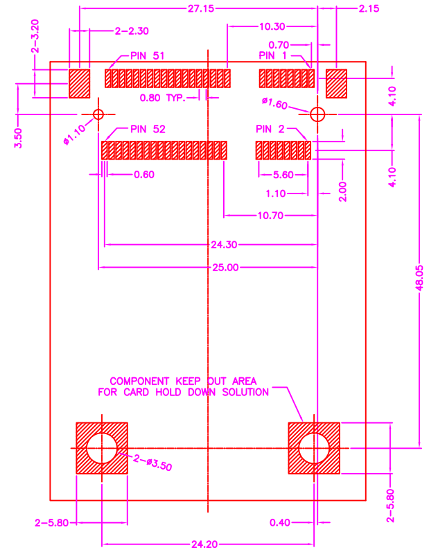
P.C.B. LAYOUT TOP VIEW ±0.05
