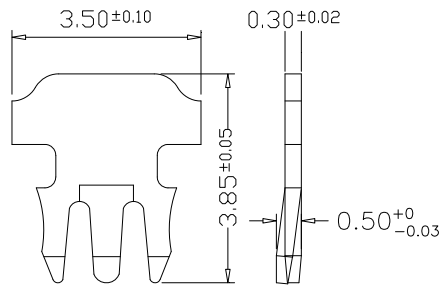
3 PRONGS FOR SOLID WIRE(S) 單芯線用三叉型金片
