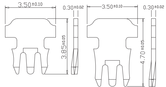
3 PRONGS FOR SOLID WIRE(S) 單芯線用三叉型金片
