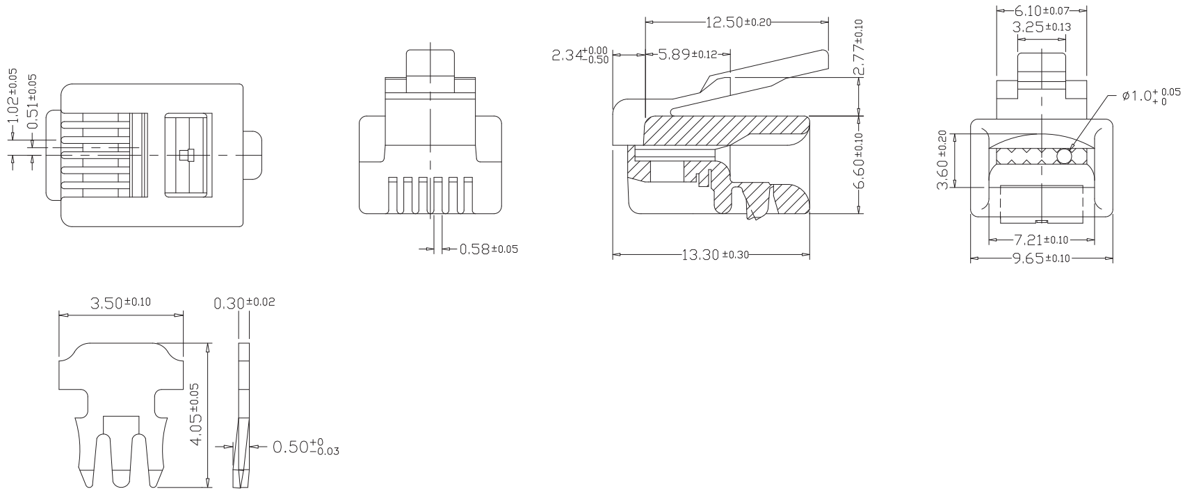
3 PRONGS FOR SOLID WIRE(S) 單芯線用三叉型片
