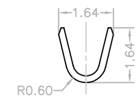
SEC:C-C
