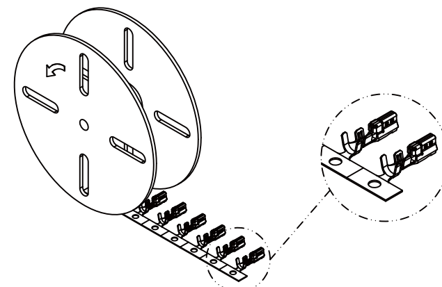
Unwind direction
