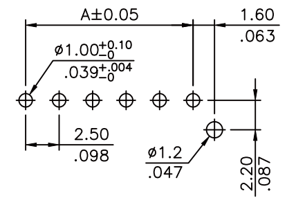
Recommended P.C. Board Layout Tolerance: ±0.05
