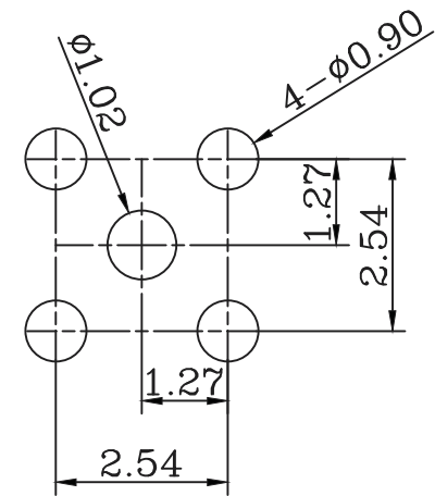
PCB MOUNT HOLES
