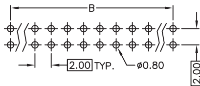
RECOMMEND P.C.B. LAYOUT BOTTOM VIEW
