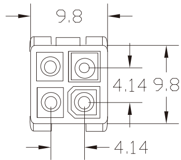
ML-P-2X02
