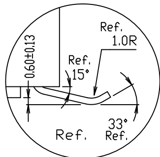
DETAIL X
