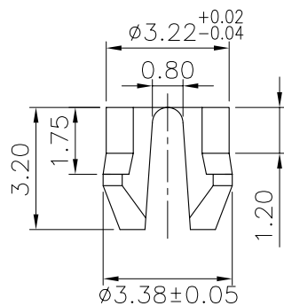
DETAIL X
