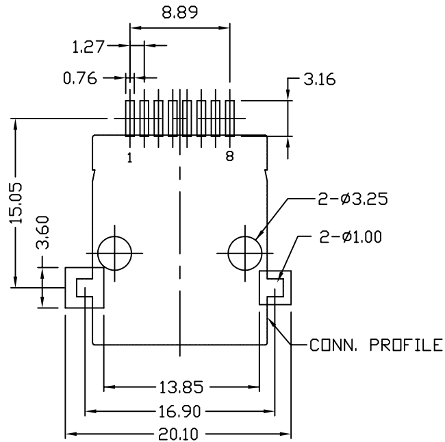
PCB LAYOUT
