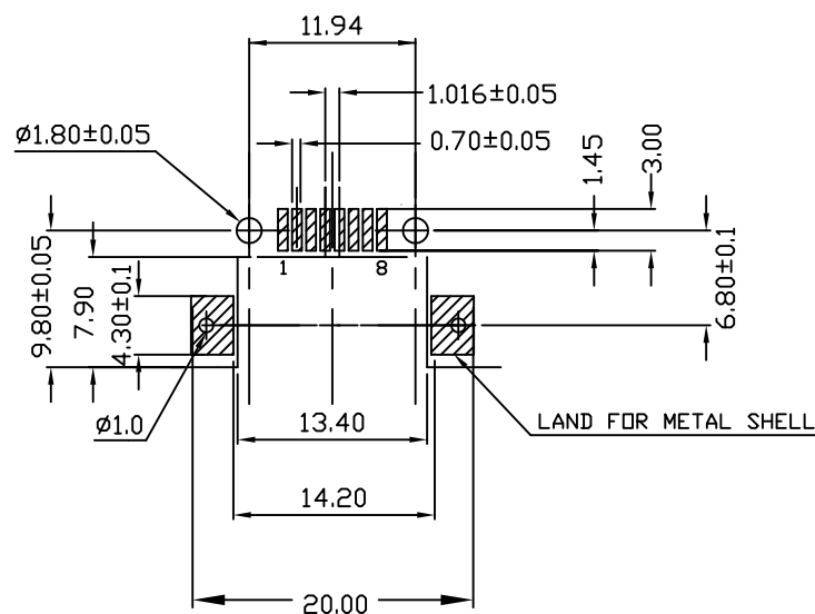
PCB LAYOUT
