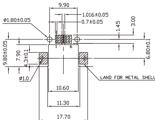
PCB LAYOUT
