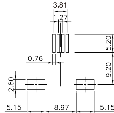
PCB LAYOUT Ref.
