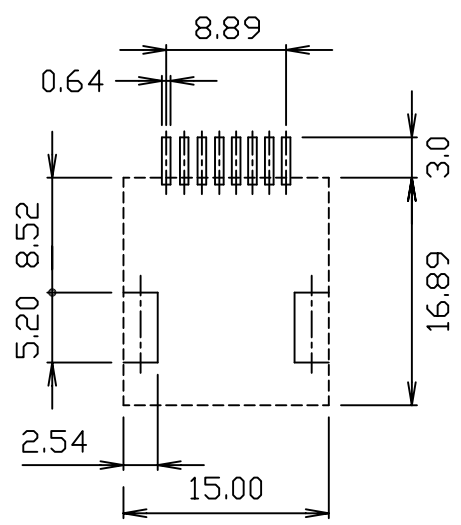
PCB LAYOUT
