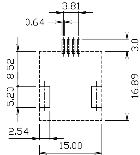
PCB LAYOUT
