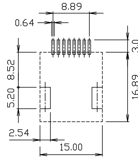
PCB LAYOUT
