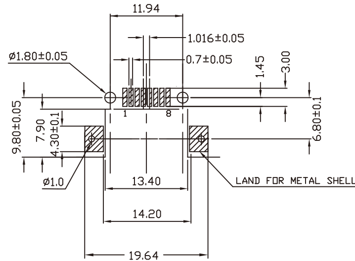
PCB LAYOUT
