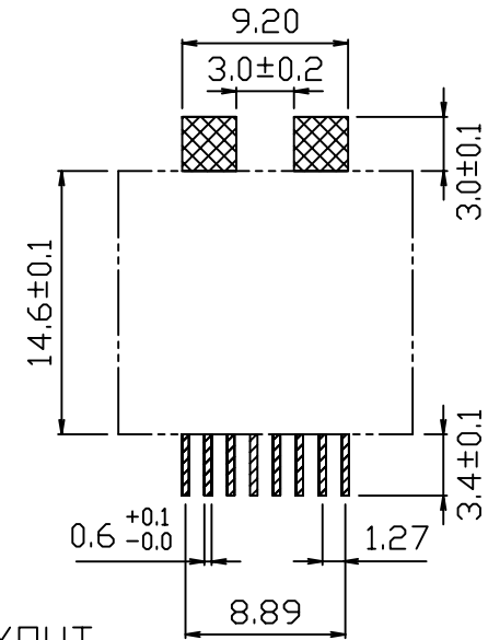
PCB LAYOUT
