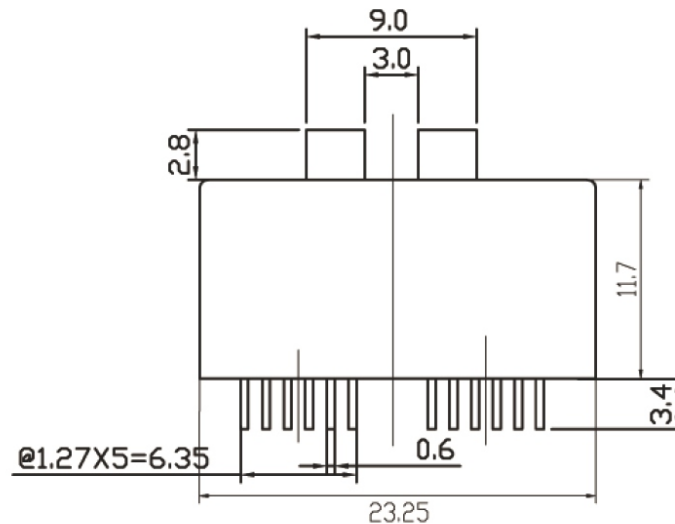
PCB LAYOUT
