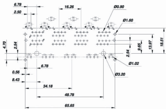
PC Layout (Top View)
