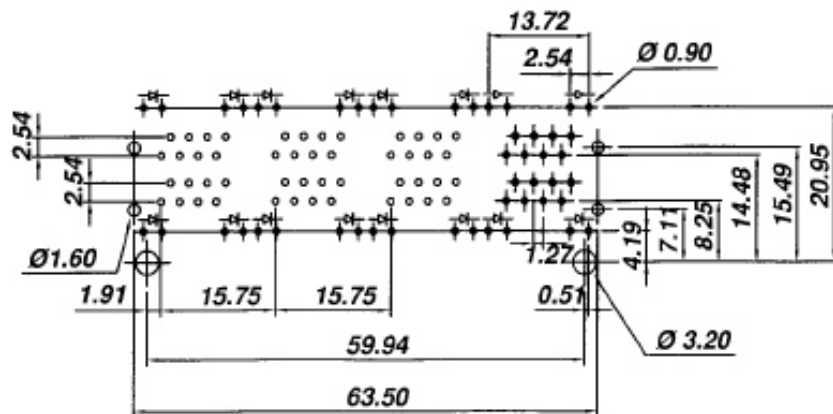
PC Layout (Top View)
