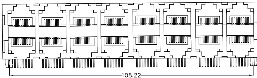
PCB LAYOUT
