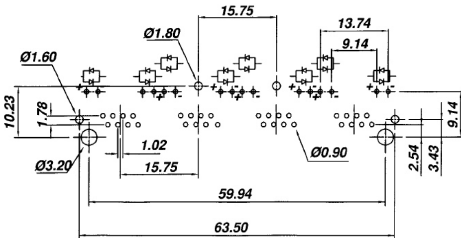
PCB LAYOUT (Top View)
