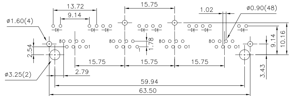
PCB LAYOUT (Ref.)
